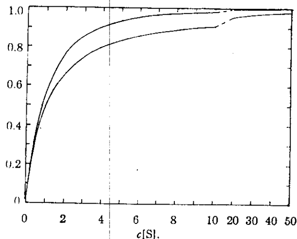
Fig. 1.—Efficiency of competition of scavenger with combination (reaction 3): lower curve is c[S]/(1 + c[S]) ; upper curve is 4/(3 + \sqrt{1 + 16/c^2[S]^2}) .
