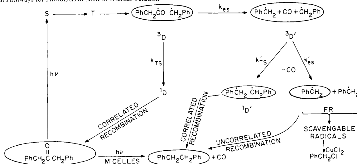
Scheme I. Pathways for Photolysis of DBK in Micellar Solution
