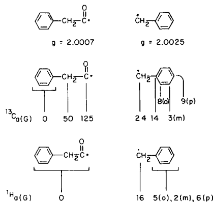
Figure 3. Relevant magnetic parameters for the \text{PhCH}_2\dot{\text{C}}\text{O}\dot{\text{C}}\text{H}_2\text{Ph} radical pair. The values for ^{13}\text{C} hyperfine coupling in the \cdot\text{CH}_2\text{Ph} radical are computed from measured proton hyperfine coupling constant according to the procedure given by: Karplus, M.; Fraenkel, G. K. J. Chem. Phys. 1961 , 35 , 1312. The other values are derived from direct ESR measurements in the literature. 9
