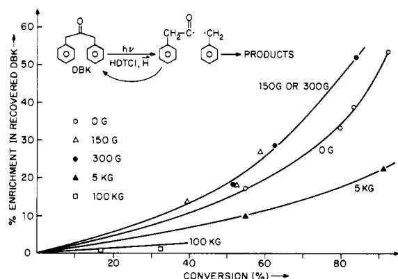
Figure 1. The percent ^{13}\text{C} enrichment at a single carbon atom of dibenzyl ketone as a function of conversion at various magnetic fields. The percent enrichment is computed from mass spectrometric data as described in the preceding paper.
