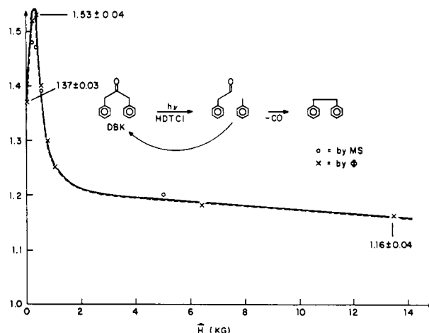
Figure 2. Variation of \alpha as a function of applied laboratory field.
