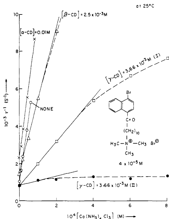
Figure 6. \tau^{-1} vs. [\text{Co}(\text{NH}_3)_6\text{Cl}_3] plots for \text{BNK-10}^+ in \text{H}_2\text{O} (O), \alpha\text{-CD} (X; 0.01 M), \beta\text{-CD} ( \Delta ; 2.5 \times 10^{-3} M), \gamma\text{-CD} ( \square ; 3.66 \times 10^{-3} M assigned to type I inclusion, and \gamma\text{-CD} ( \bullet ; 3.66 \times 10^{-3} M assigned to type II inclusion) at 25 °C. [\text{BNK-10}^+] = 4 \times 10^{-5} M.
