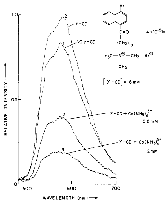
Figure 2. Phosphorescence spectra of BNK-10 ^+ in the presence of \gamma -CD and \text{Co}(\text{NH}_3)_6\text{Cl}_3 at 25 ^\circ\text{C} ; [BNK-10 ^+ ] = 4 \times 10^{-5} M. Curve 1, in \text{H}_2\text{O} ; curve 2, [ \gamma -CD] = 8 mM; curve 3, [ \gamma -CD] = 8 mM, [ \text{Co}(\text{NH}_3)_6^{3+} ] = 0.2 mM; curve 4, [ \gamma -CD] = 8 mM, [ \text{Co}(\text{NH}_3)_6^{3+} ] = 2 mM.
