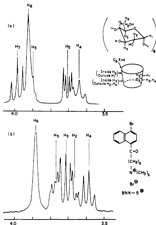
Figure 1. 300-MHz ^1\text{H} NMR spectra of \gamma -cyclodextrin in the (a) absence and (b) presence of BNK-5 ^+ in \text{D}_2\text{O} .
