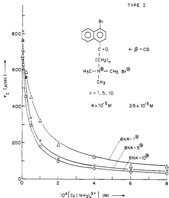
Figure 7. \tau^{-1} vs. [\text{Co}(\text{NH}_3)_6^{3+}] plots for \text{BNK-1}^+ and \beta\text{-CD} ( \Delta ), \text{BNK-5}^+ and \beta\text{-CD} (X), and \text{BNK-10}^+ and \beta\text{-CD} (O) systems at 25 °C. [\text{BNK-}n^+] = 4 \times 10^{-5} M; [\beta\text{-CD}] = 2.5 \times 10^{-3} M.
