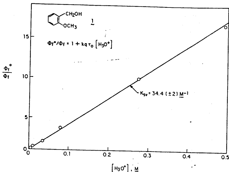
Fig. 4. Stern-Volmer plot of \Phi_f^0/\Phi_f vs. [H_3O^+] for 2-methoxybenzyl alcohol (1).
