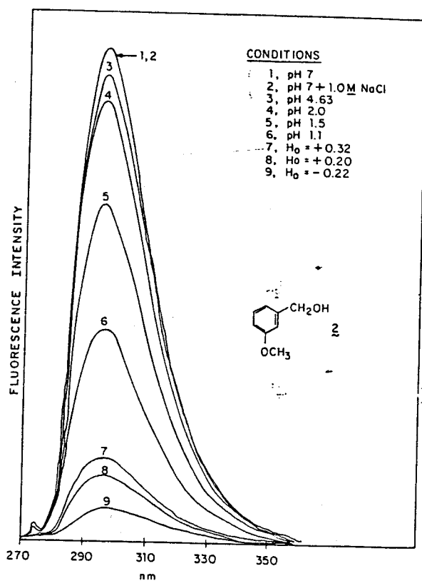
Fig. 1. Dependence of fluorescence intensity on medium acidity (aqueous HCl and H_2SO_4 ) for 3-methoxybenzyl alcohol ( 2 ) (excitation wavelength, 275 nm; substrate concentration, 10^{-4} M).
