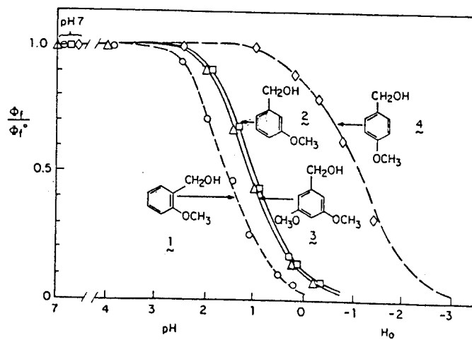
Fig. 2. Fluorescence quenching as a function of medium acidity for benzyl alcohols 1 - 4. \phi_f^0 is defined as the fluorescence intensity at pH 7 ( H_0 is the Hammett acidity function scale).
