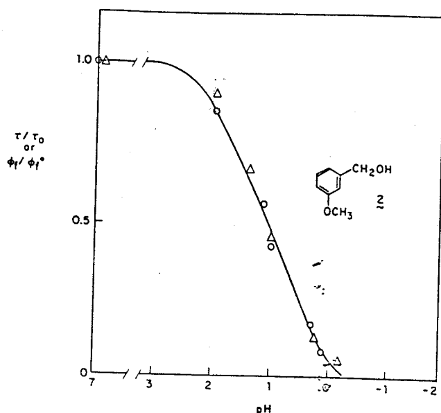
Fig. 3. Plot of \tau/\tau_0 (O) and \phi_f/\phi_f^0 ( \Delta ) for 3-methoxybenzyl alcohol (2) as a function of medium acidity. \tau_0 and \phi_f^0 are the lifetime and the fluorescence quantum yield in pH 7. The ratios are normalized to unity in pH 7.
