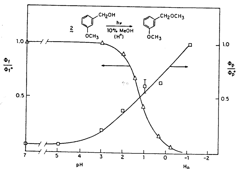
Fig. 5. Fluorescence quenching by acid and relative quantum efficiency for methyl ether formation for 3-methoxybenzyl alcohol (2). \Phi_p^\circ is the yield of methyl ether at H_0 = -1 , normalized to unity. Absolute quantum yields were not measured (fluorescence quenching experiments were performed in wholly aqueous solutions).
