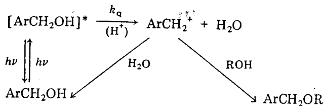
Fig. 6. Proposed reaction mechanism for 1 - 3.
