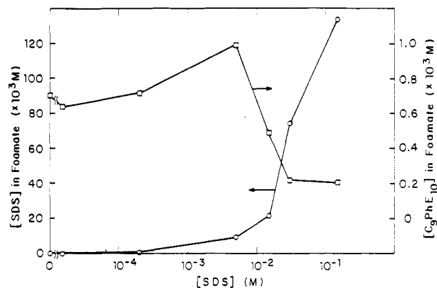
Figure 6. Foamate concentrations of SDS and C_9PhE_{10} as a function of [SDS] .
