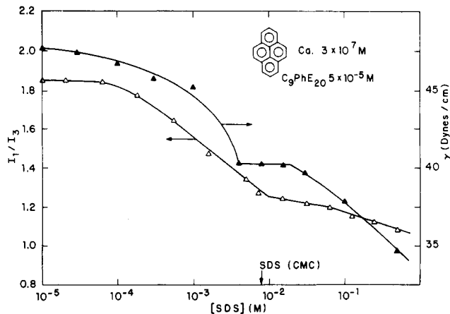
Figure 4. Correlation between the plots of I_1/I_3 vs. [SDS] and of \gamma vs. [SDS] with C_9PhE_{20} fixed at 5.0 \times 10^{-5} M.
