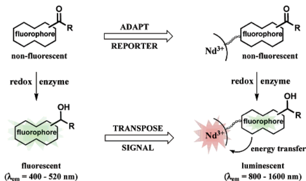
Figure 1. The concept of adapting a fluorogenic redox reporter (left) to a NIR emitting format by the incorporation of lanthanide ions (right).
