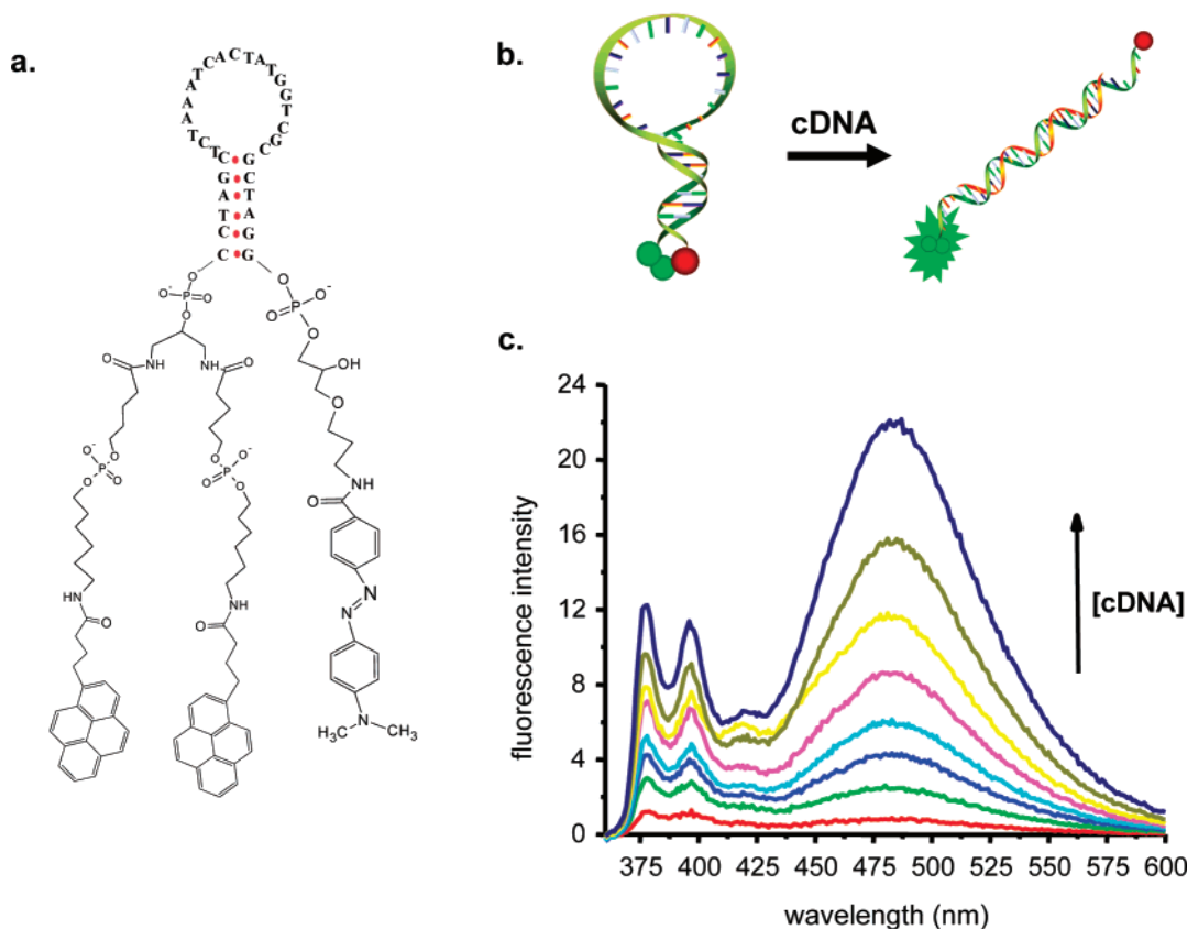
Figure 1. (a) Structural representation of MB-2P with pyrene monomers labeled to dual 5' linker chains and DABCYL molecule labeled to 3' chain. (b) Schematic of MB-2P hybridization with complimentary target. (c) Emission spectra of 1 μM MB-2P with increasing concentrations of cDNA in buffer solution. The excimer signal increases upon addition of cDNA and reaches maximum intensity at 1 equiv of target (1 μM cDNA). (Buffer: 20 mM Tris-HCl, 25 mM NaCl, 5 mM MgCl 2 , pH: 7.4.)
