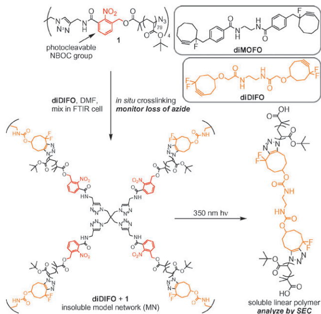
Scheme 1 Structures of star polymer 1 , diMOFO, diDIFO, MN from diDIFO and 1 , and the corresponding linear polymer photodegradation product. To clearly depict their location in the MN structure, photodegradable NBOC groups are shown in red and diDIFO is shown in orange.
