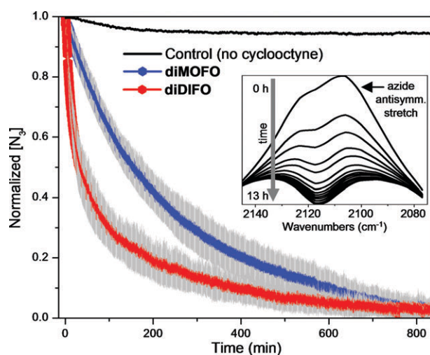
Fig. 1 Average decay curves for the loss of azide during gelation between 1 and diMOFO or diDIFO as monitored by FTIR. Experiments were performed in triplicate with error bars shown in grey. Inset shows the azide antisymmetric stretch region of the FTIR spectrum at different intervals during a typical gelation experiment with diDIFO .
