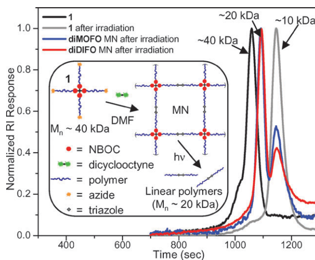
Fig. 2 SEC traces of 1 before and after photocleavage, and of the photodegradation products of diMOFO and diDIFO derived MNs. Inset shows schematic of crosslinking depicting the conversion of 1 to a MN and finally to linear polymers having M_n \approx 0.5 that of 1 .
