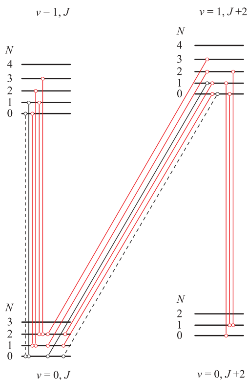
FIG. 1. Diagram of the observed IR transitions. The diagram describes para - \text{H}_2 states if the rotational quantum number J = 0 and ortho - \text{H}_2 states if J = 1 . Vibrational quantum number is \nu and translational quantum number is N . The additional structure of energy levels E_{JNL\Lambda}^{\nu} due to quantum numbers L and \Lambda is not shown. Dashed lines are forbidden transitions, and black lines are the only transitions that are observable at low temperature (see also Fig. 2 in Ref. 6).
