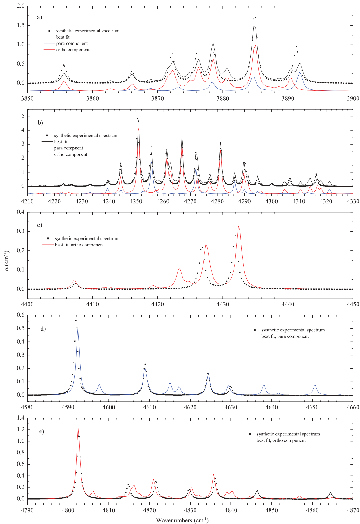
FIG. 7. Synthetic experimental absorption spectra of \text{H}_2@C_{60} at 200 K (dots) together with the fit result, \text{FWHM} = 1 \text{ cm}^{-1} . The total absorbance \alpha is the sum of para and ortho components, shifted in vertical direction for clarity and shown separately in panels (a) and (b), where both components have a significant contribution. Above 4400 \text{ cm}^{-1} only para , panel (d), or ortho , panels (c) and (e), components of the fit are shown, as the other component does not have any contribution.
